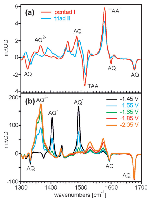
Figure 1. a) Transient IR difference spectra measured after excitation of 1 mM solutions of pentad I and triad II in dry, de-aerated \text{CD}_3\text{CN} at 415 nm with laser pulses of approximately 100 fs duration. The excitation pulse energy was 2 \mu\text{J} , the spectra were recorded 0.5 ns after excitation. b) IR difference spectra measured after application of different potentials to a 5 mM solution of 9,10-anthraquinone in \text{CD}_3\text{CN} . The IR spectrum measured prior to application of any potential served as a baseline. Potentials are reported versus \text{Fc}^+/\text{Fc} .
