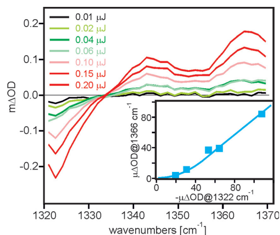
Figure 3. Dependence of the AQ bleach at 1322\text{ cm}^{-1} and the \text{AQ}^{2-} absorption band at 1366\text{ cm}^{-1} on the excitation pulse energy. The data have been averaged over various time points ranging from 1 to 100 ns to enhance the signal-to-noise ratio. The inset shows the change in optical density (OD) at 1366\text{ cm}^{-1} compared to that at 1322\text{ cm}^{-1} , which reports on the bleaching of AQ and as such is used as an internal standard (which is free of the uncertainty originating from, for example, the alignment of the spatial overlap between pump- and probe pulse). The data are fitted to a quadratic function up approximately 0.03\text{ }\mu\text{J} , and to a linear function beyond.
