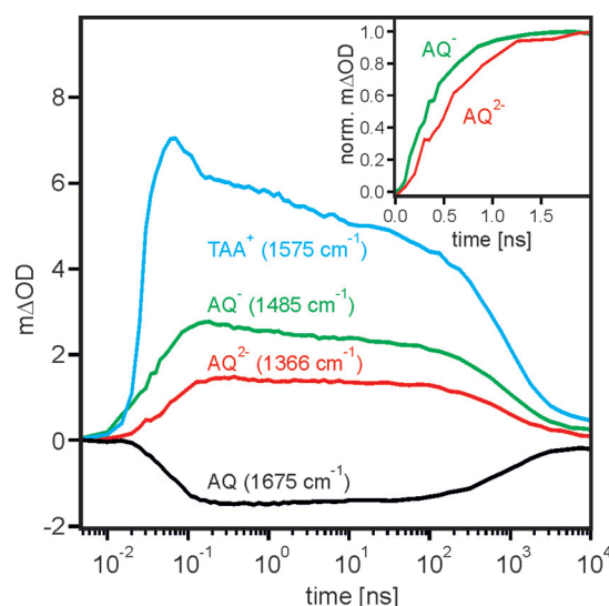
Figure 2. Temporal evolution of some of the key signals observed for pentad I in Figure 1. The inset shows the normalized early rise of the bands originating from \text{AQ}^- and \text{AQ}^{2-} .
