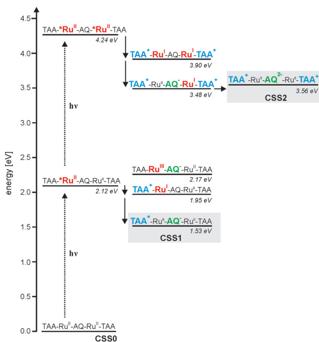
Scheme 2. Energy-level diagram established on the basis of electrochemical and UV/Vis data (Supporting Information page S11). Energy estimates are accurate to approximately \pm 0.1\text{ eV} .
